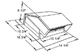
Sloped Roof Cap
